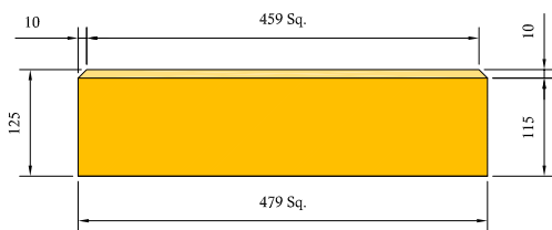
Under Plinth
