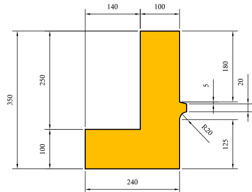
Architrave (Section)
