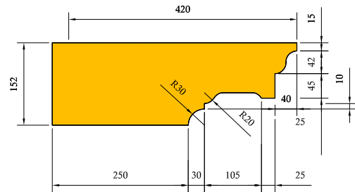
Lower Cornice
