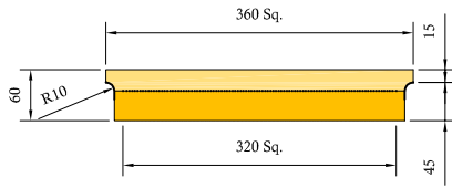
Top Piece
