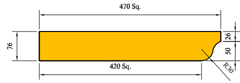
Upper Cornice
